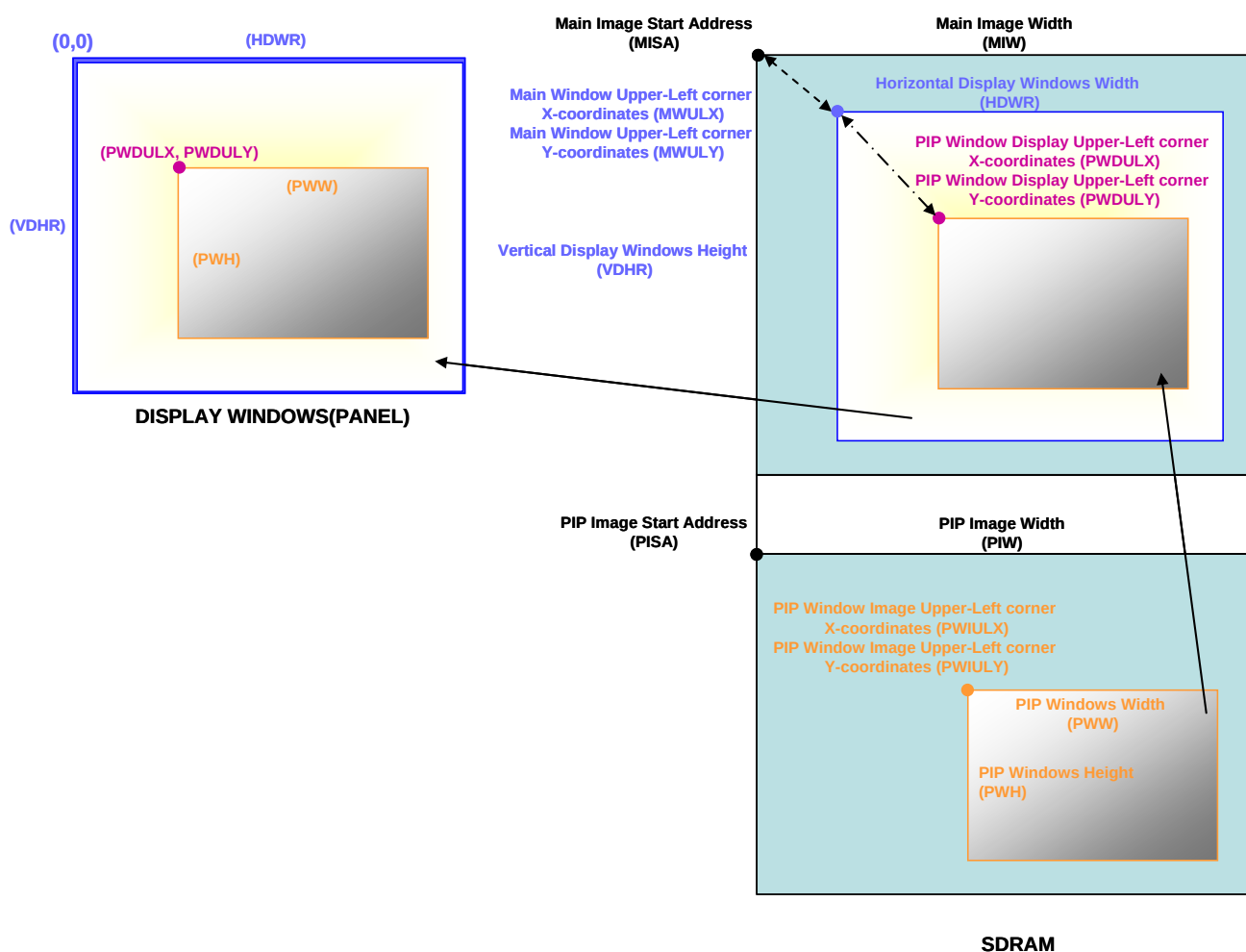
Figure 20-2 : LCD Display
